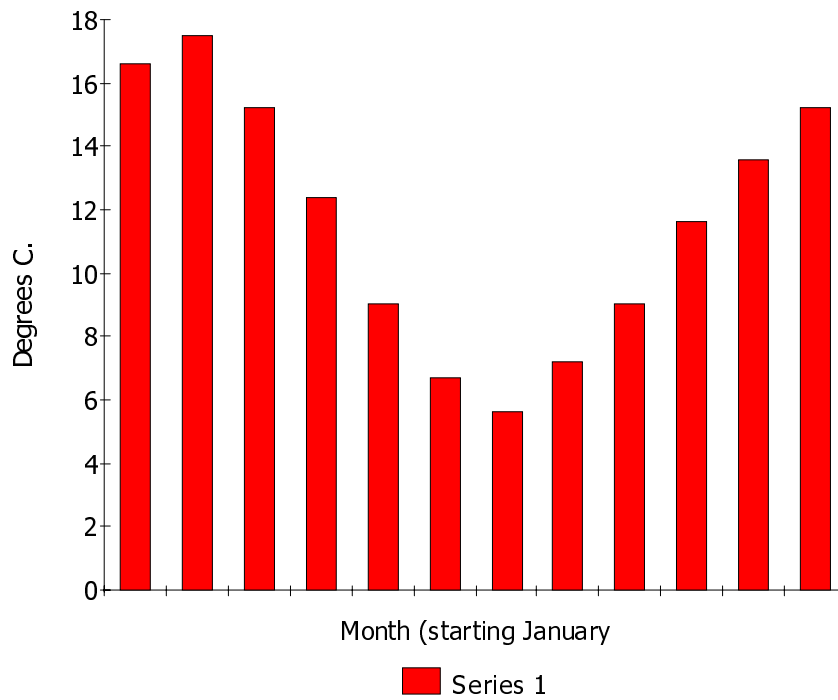
Average maximum temperatures
