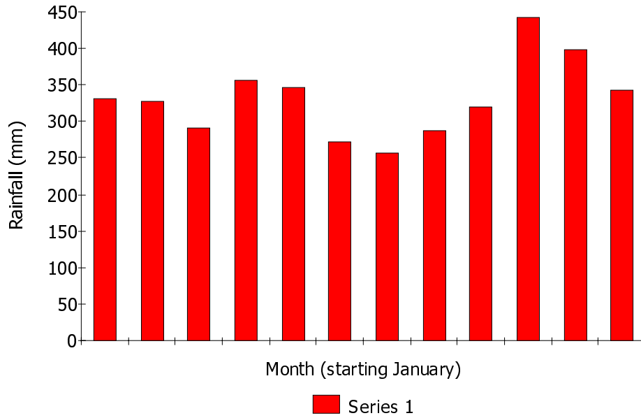
Monthly Rainfall at Arthur's Pass
